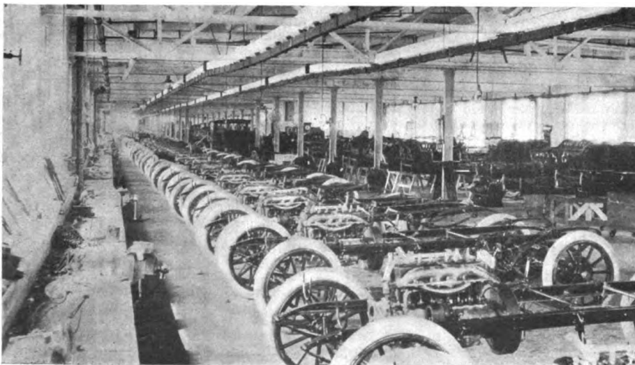
Assembling Department of the E-M-F Factory Showing Completed Cars.
